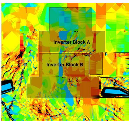
Topography map with tracker layout for Southeast U.S. project site.
