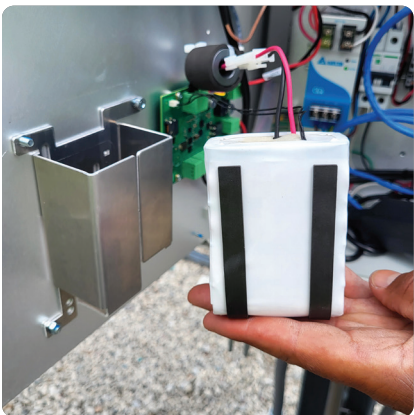
Panasonic Lithium Ion Battery, 8 Cell
